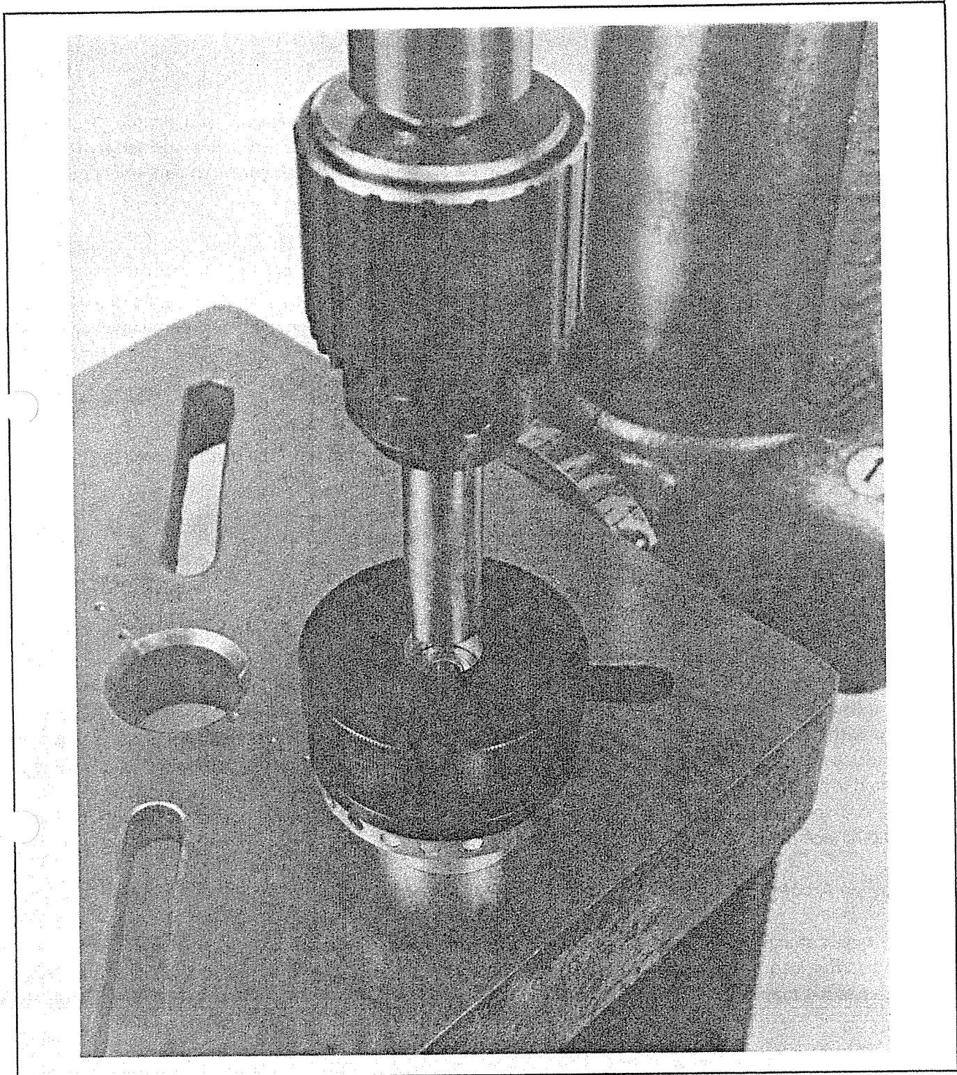
Figure 9-2. Bearing Remover
