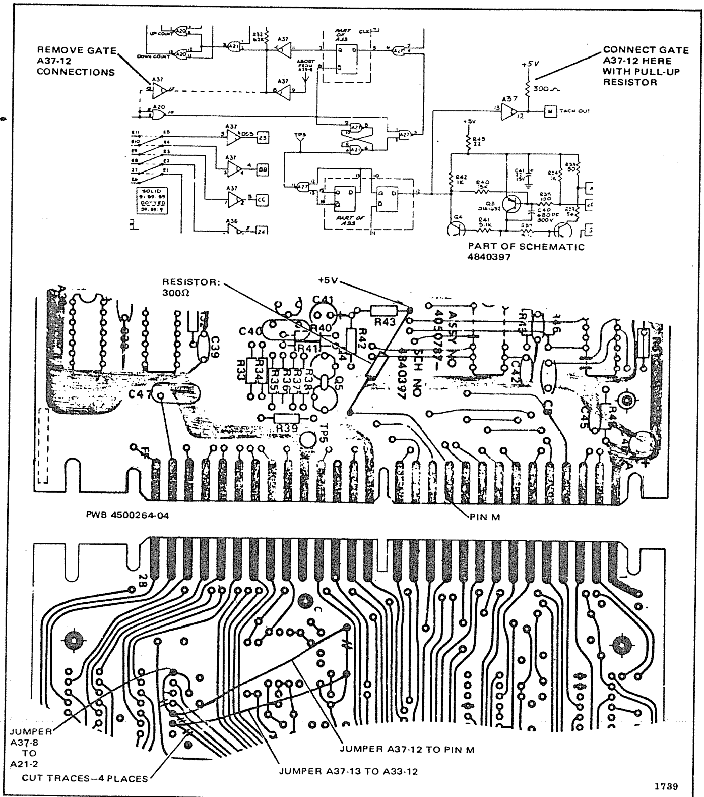
Figure 2-1. Modification to ATR-100 Logic and Tape Timer PWA
